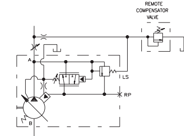
PUMP WITH REMOTE PRESSURE CONTROL
