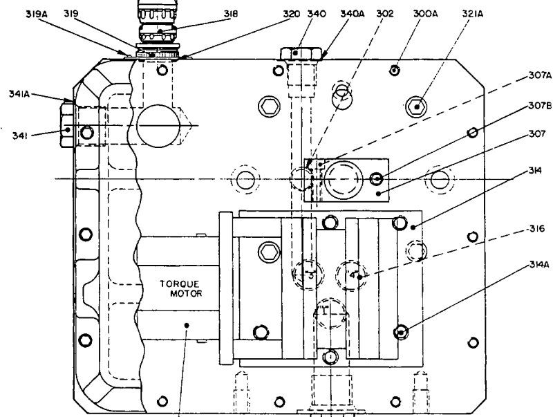
VIEW B-B W/O COVER (WITH 2.00" SERVO VALVE)
