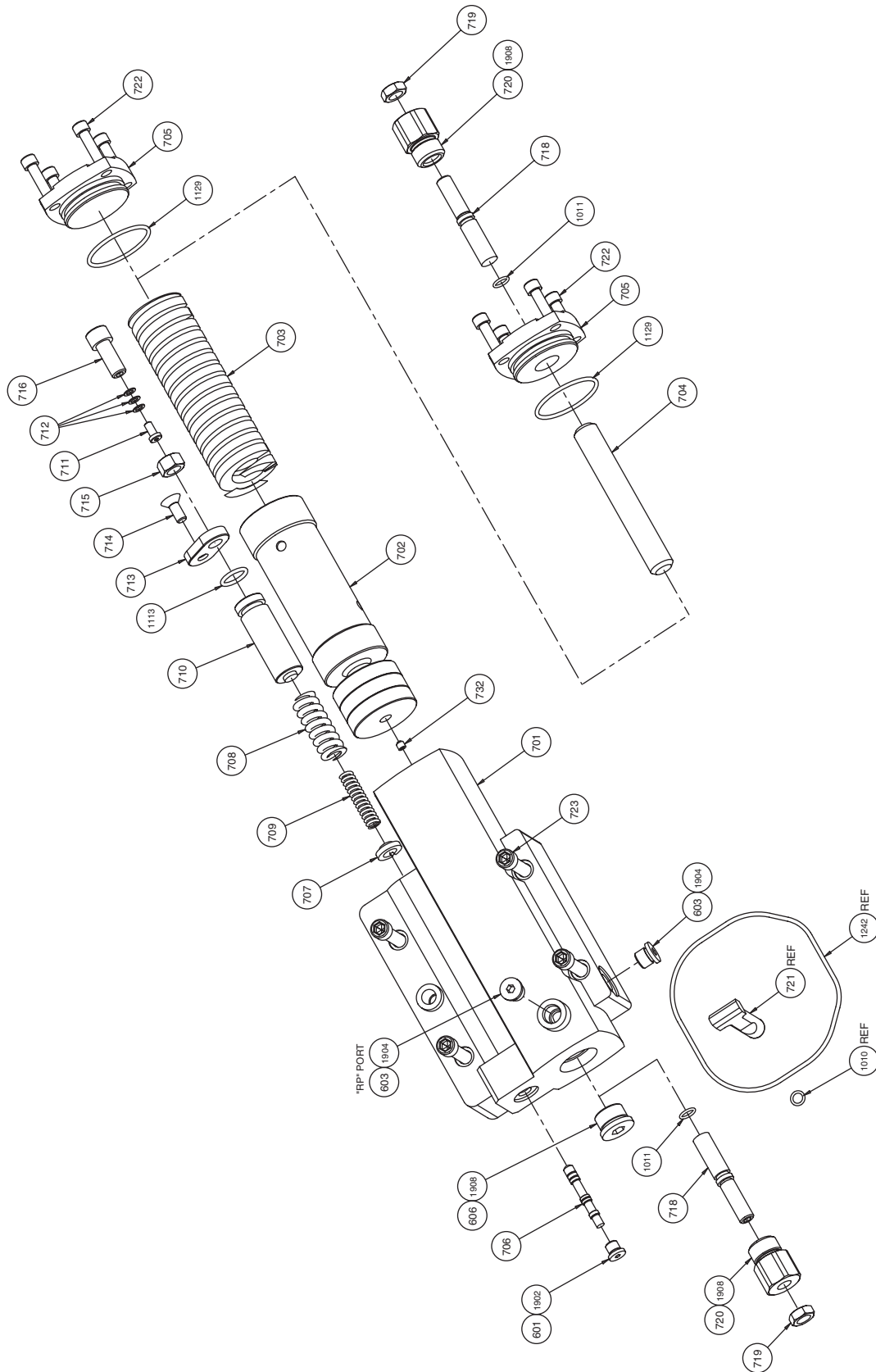
Figure 9. Exploded Parts Drawing for "P-1NN" and "P-LNN" Control (519975-301 sheet 2)
