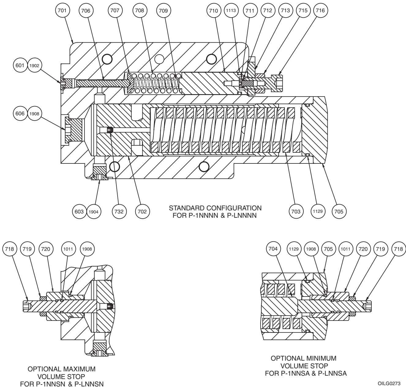
Figure 8. Parts Drawing for "P-1NN" and "P-LNN" Control (519975-301 sheet 1)
