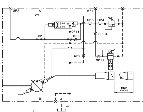
HYDRAULIC CIRCUIT
